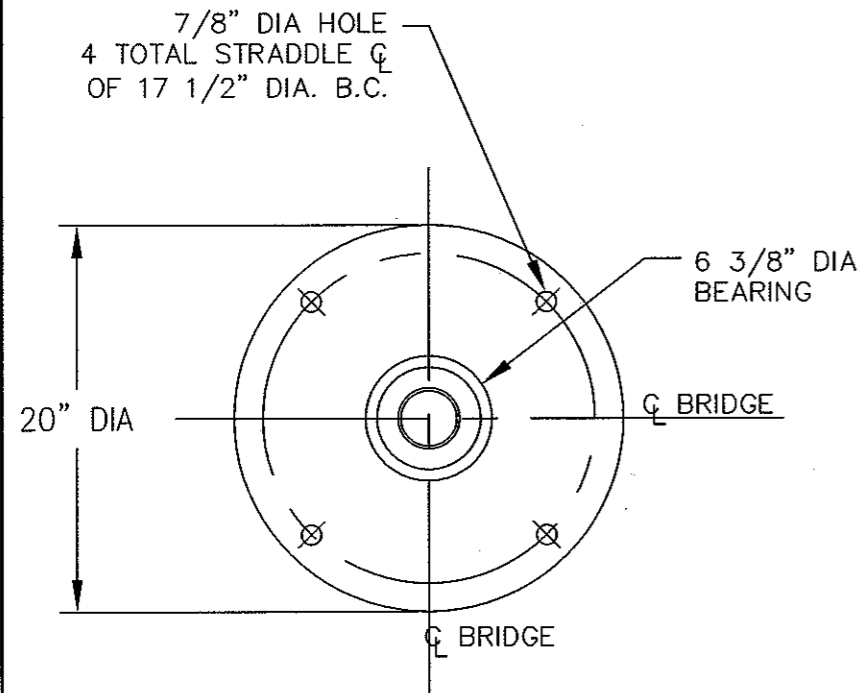
MOUNTING FLANGE
