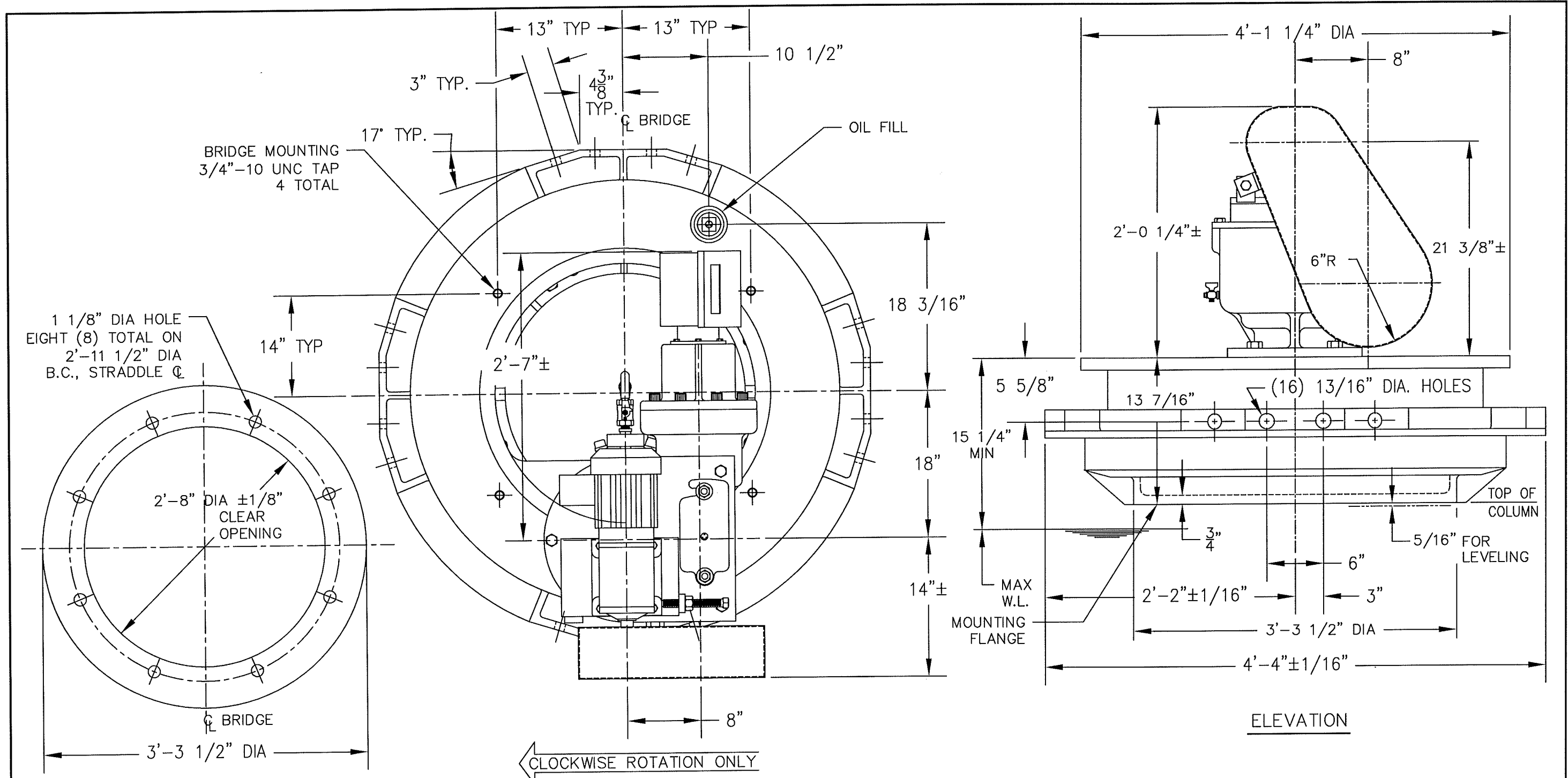
MOUNTING FLANGE
